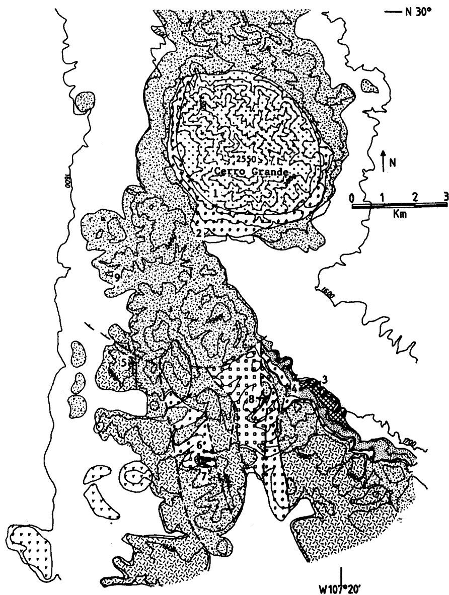
Fig. 2. Generalized geologic map of the Cerro Grande region, San Buenaventura. Contour lines drawn every 100 m, numbers indicate sample location (Table 1) (for legend, see Fig. 3).
