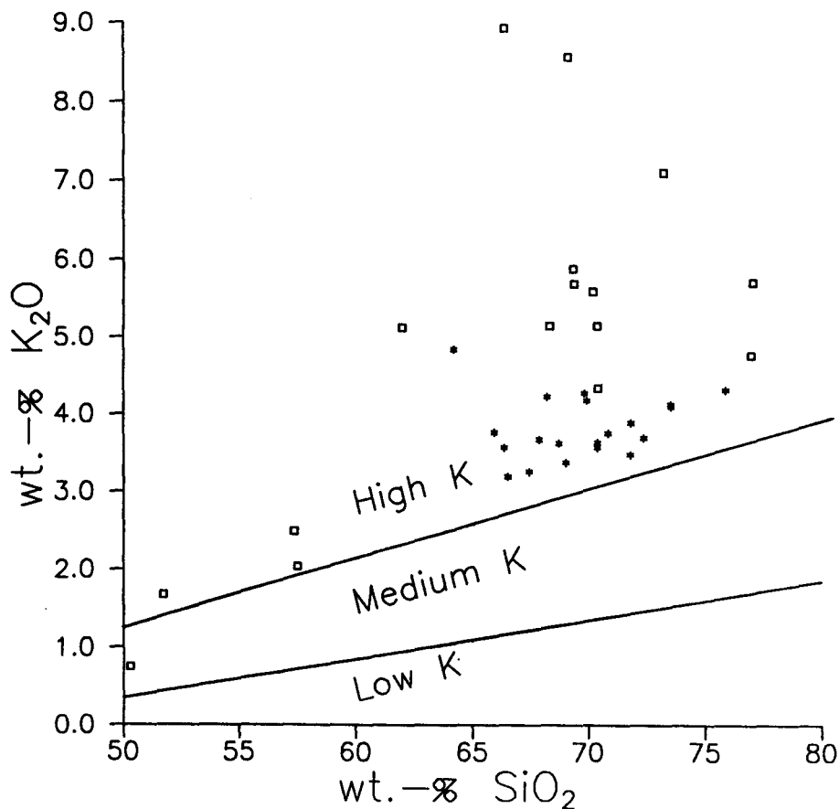
Fig. 8. Harker-type variation diagram for \text{K}_2\text{O} ; boundary lines between low-, medium and high K after Gill (1981); open squares depict Buenaventura samples, stars El Divisadero samples.
