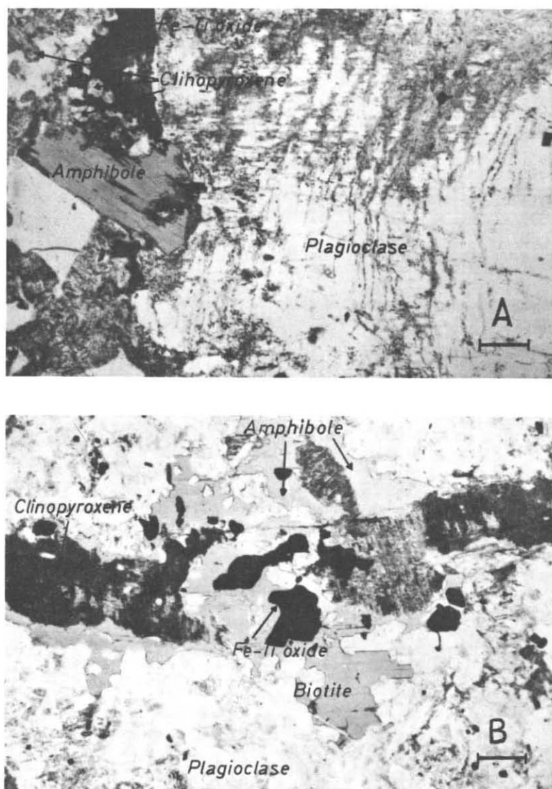
Fig. 7. Photomicrographs of plagiogranitoid sample 87/3-1; scale bar is 2.5 mm.
